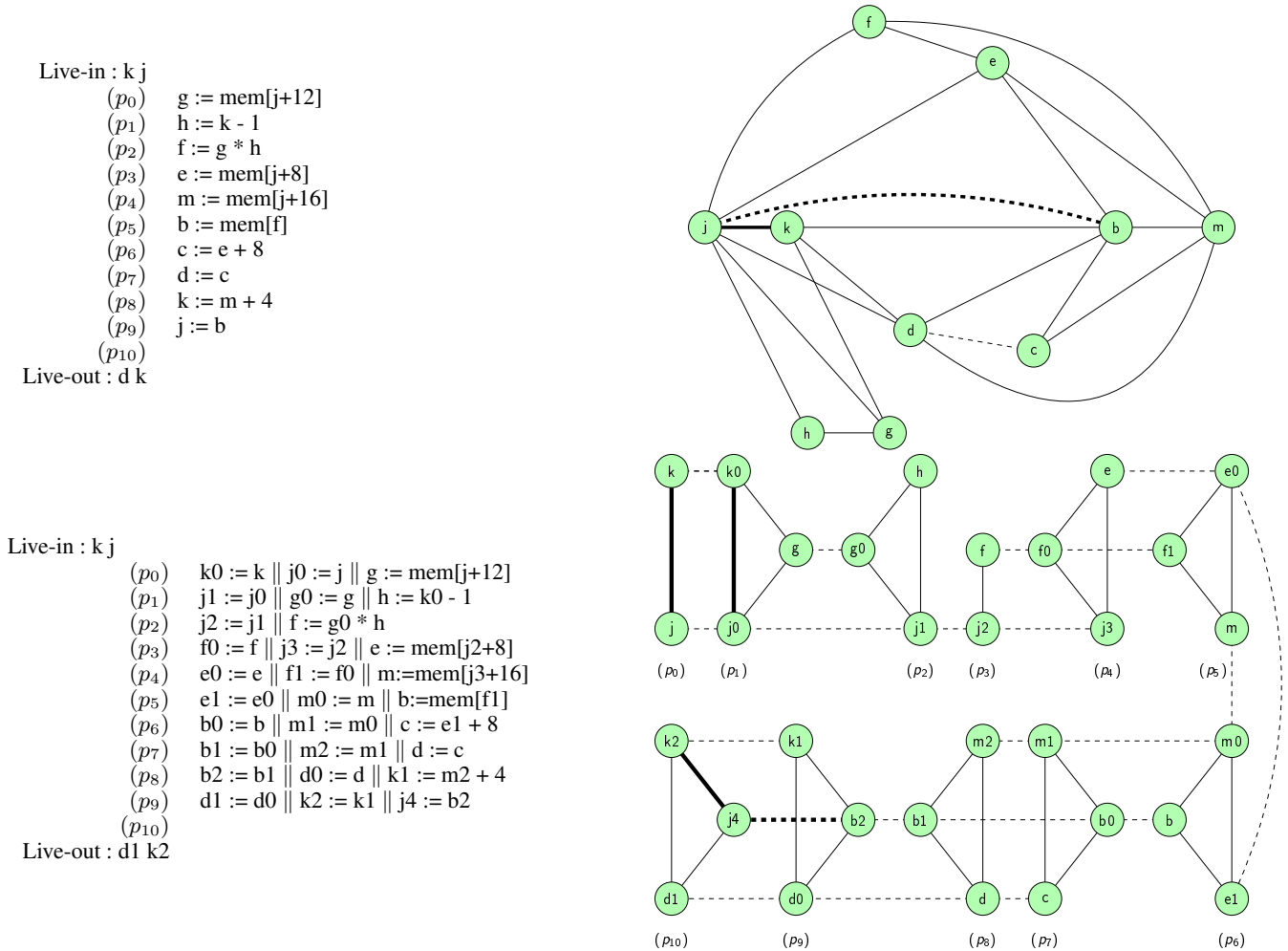
Figure 2. A small program and its interference graph (top). Full edges are interference edges. Affinity edges are dashed edges. The same program after extreme live-range splitting and its split interference graph (bottom). The weights of affinity edges are omitted in the Figure. The program points (p 0 ) . . . (p 10 ) of both programs are shown in the Figure.
